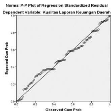
Figure 1. Results of the P-Plots Data Normality Test
